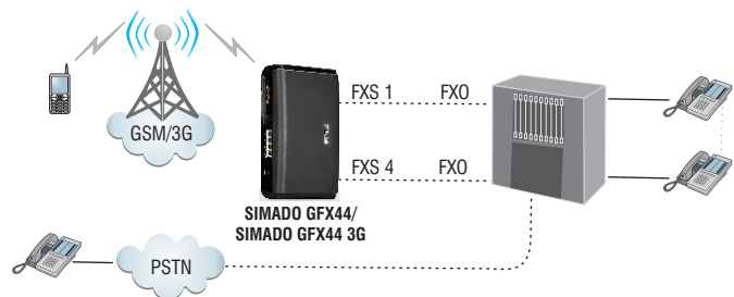
FXS with PBX (FXO) Application
